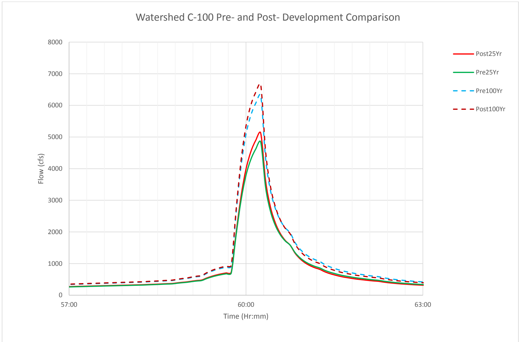
C.1 FIGURE: WATERSHED C-100 PRE- AND POST-DEVELOPMENT HYDROGRAPH
