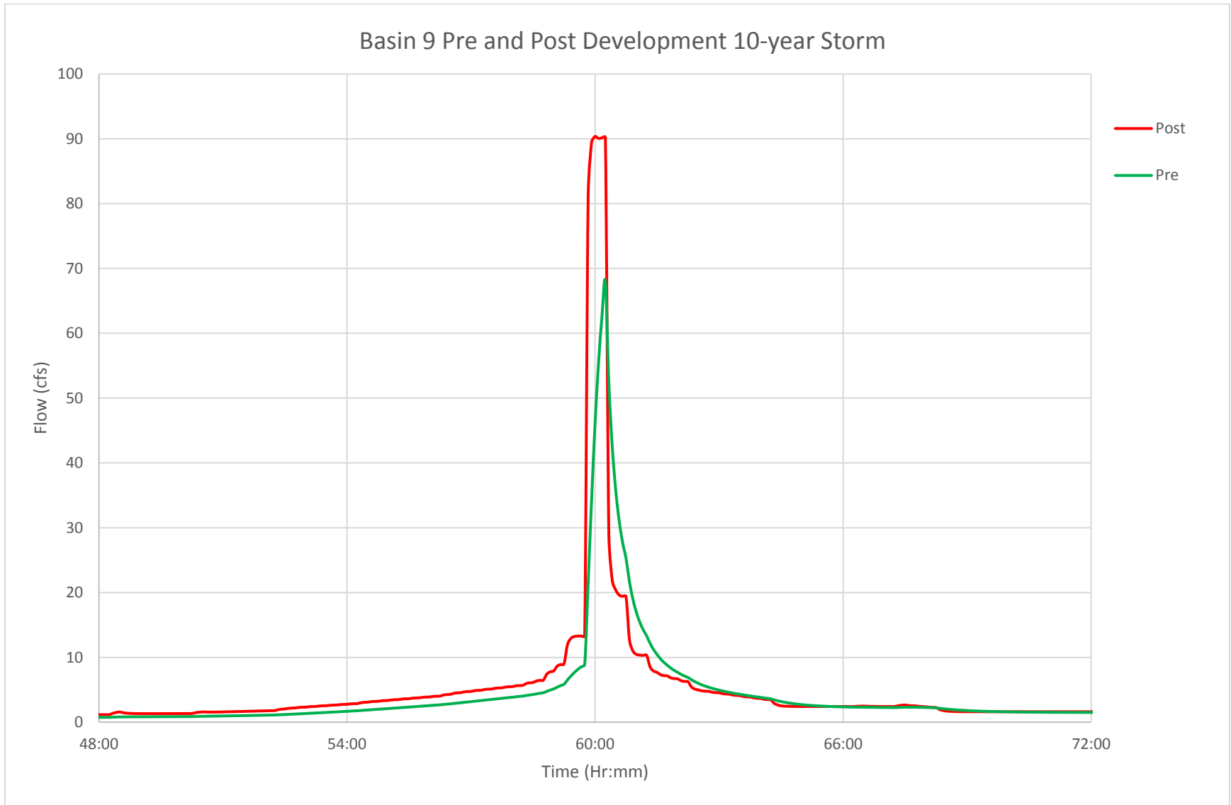
M.1 FIGURE: BASIN 9 PRE- AND POST-DEVELOPMENT HYDROGRAPH, 10-YEAR STORM
