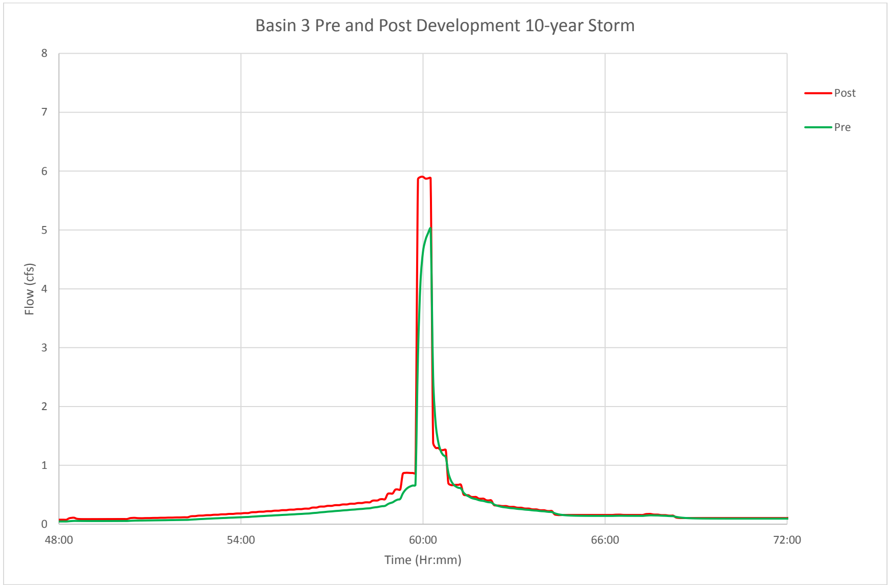
G.1 FIGURE: BASIN 3 PRE- AND POST-DEVELOPMENT HYDROGRAPH, 10-YEAR STORM
