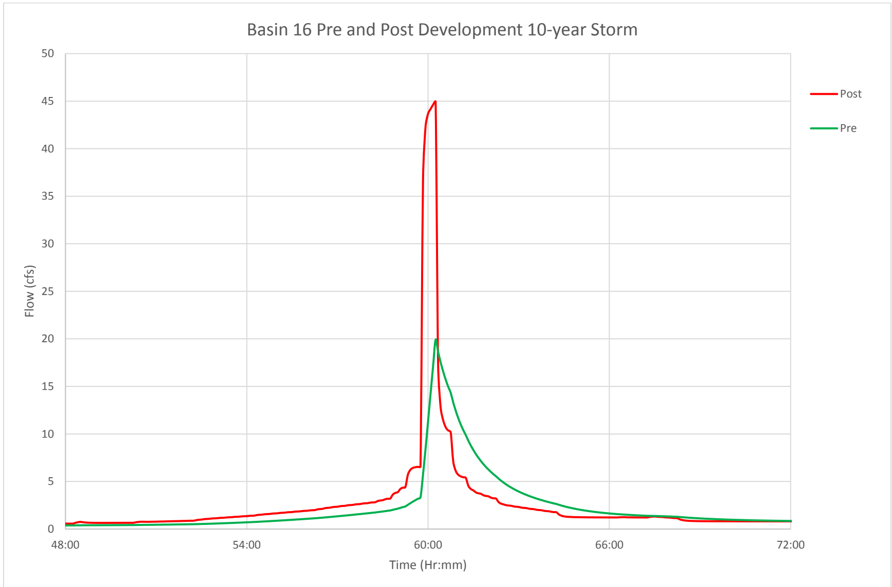
T.1 FIGURE: BASIN 16 PRE- AND POST-DEVELOPMENT HYDROGRAPH, 10-YEAR STORM
