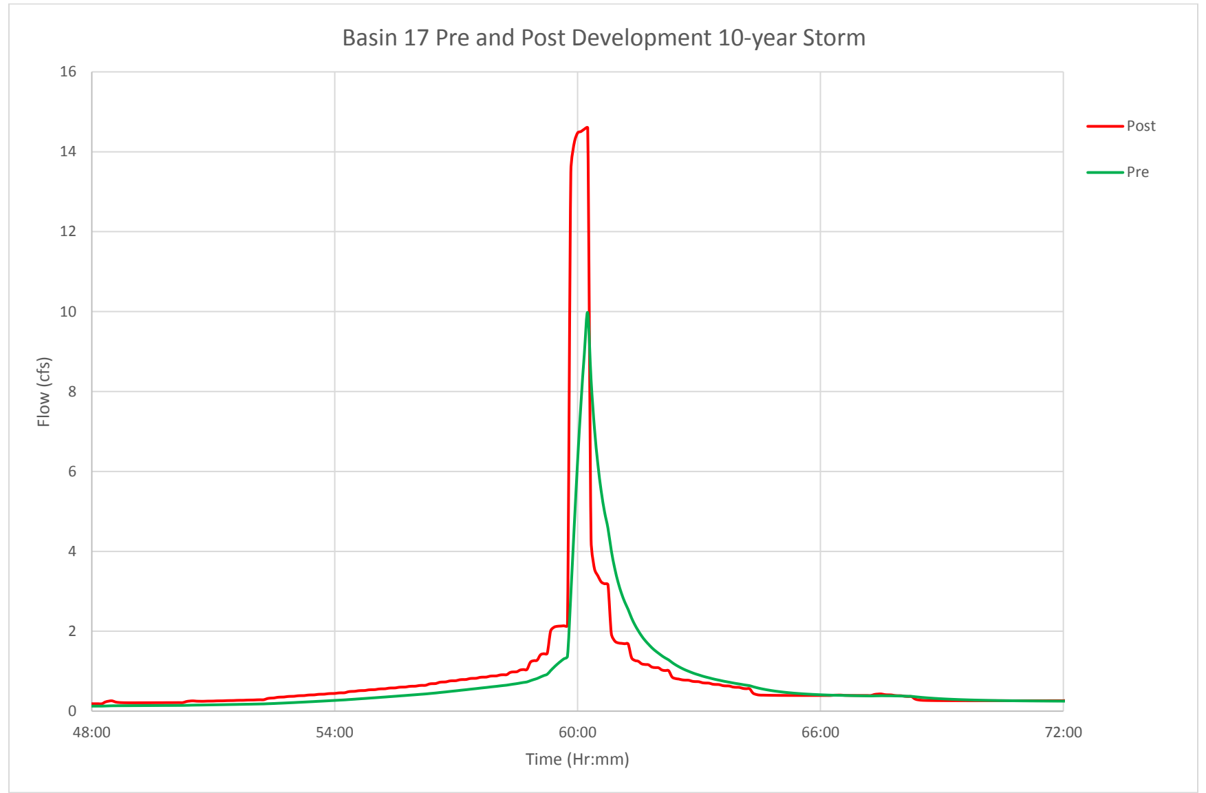
U.1 FIGURE: BASIN 17 PRE- AND POST-DEVELOPMENT HYDROGRAPH, 10-YEAR STORM
