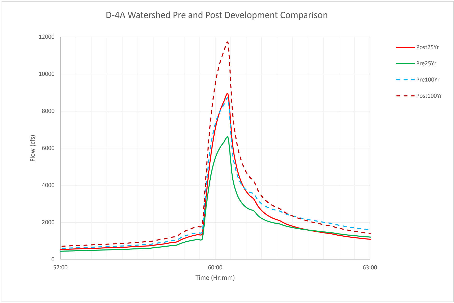
D.1 FIGURE: WATERSHED D-4A PRE- AND POST-DEVELOPMENT HYDROGRAPH
