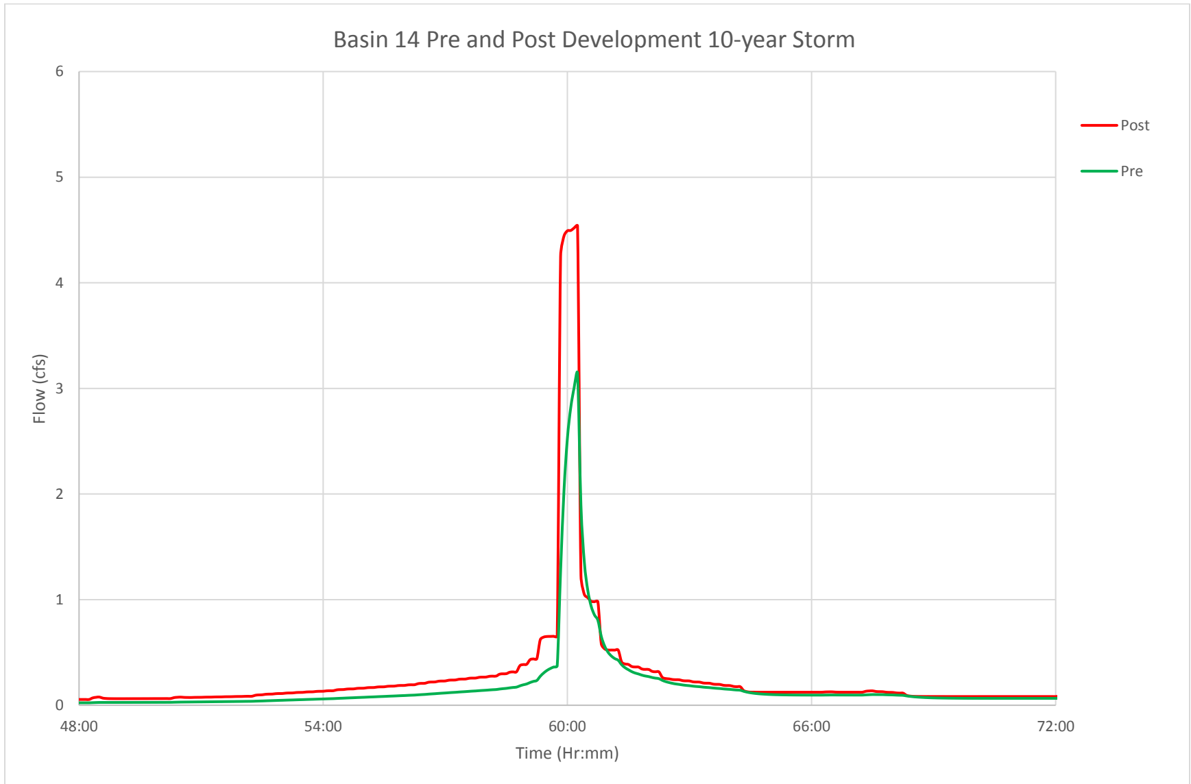
R.1 FIGURE: BASIN 14 PRE- AND POST-DEVELOPMENT HYDROGRAPH, 10-YEAR STORM
