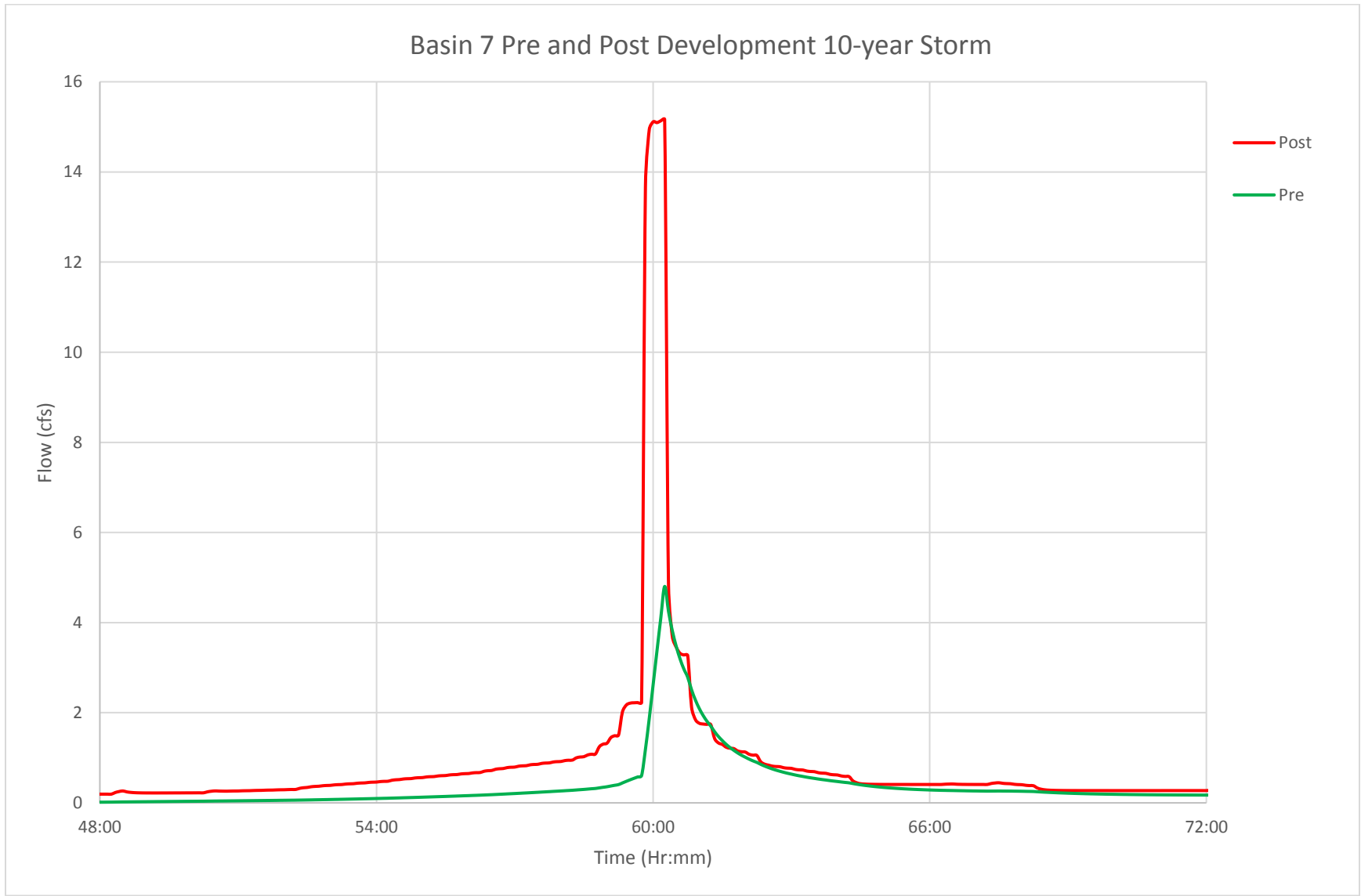
K.1 FIGURE: BASIN 7 PRE- AND POST-DEVELOPMENT HYDROGRAPH, 10-YEAR STORM
