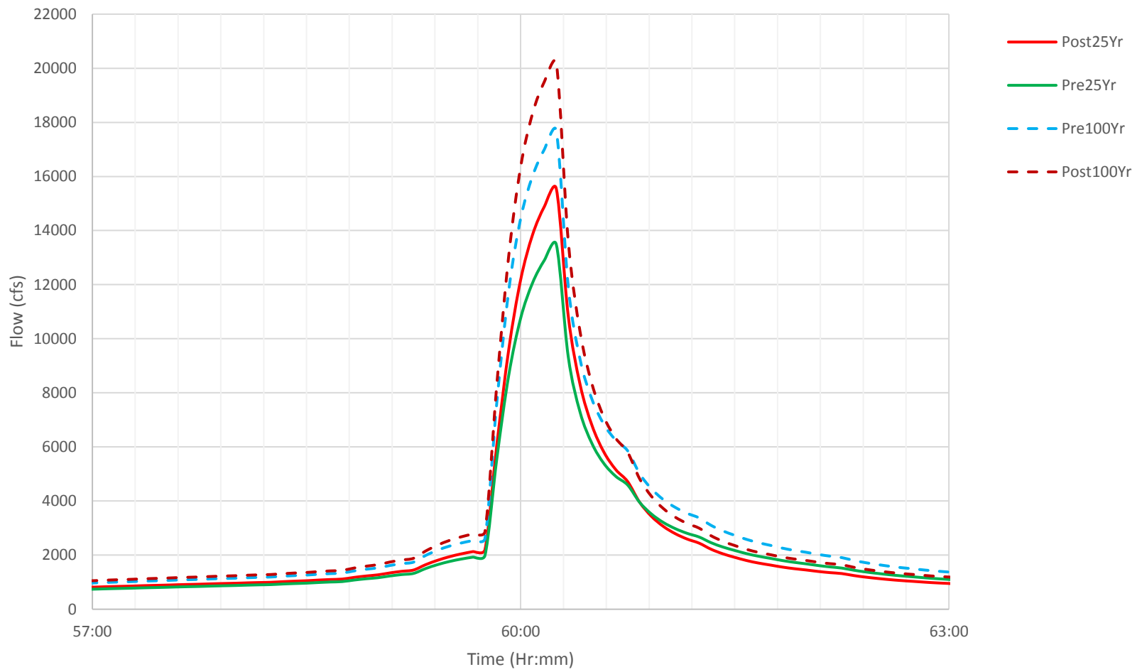
Figure 6.1 – Watershed C-1 Hydrograph
