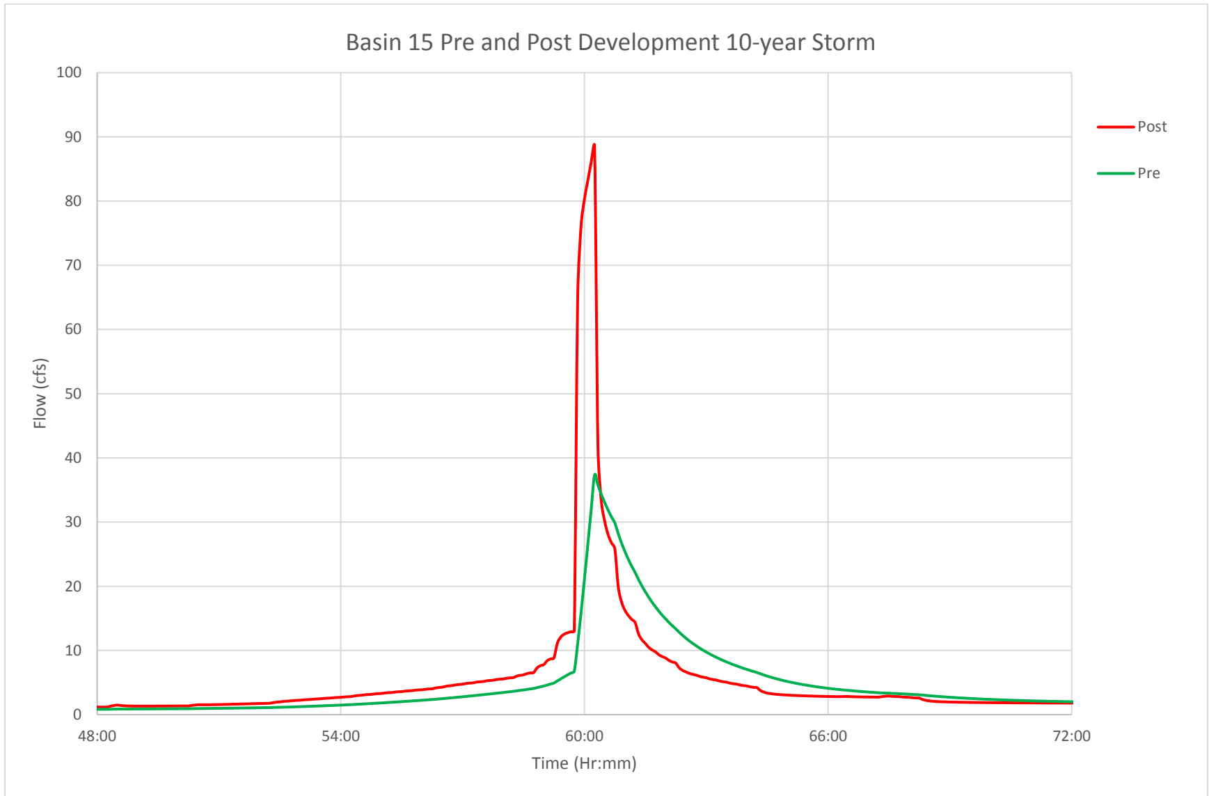
S.1 FIGURE: BASIN 15 PRE- AND POST-DEVELOPMENT HYDROGRAPH, 10-YEAR STORM
