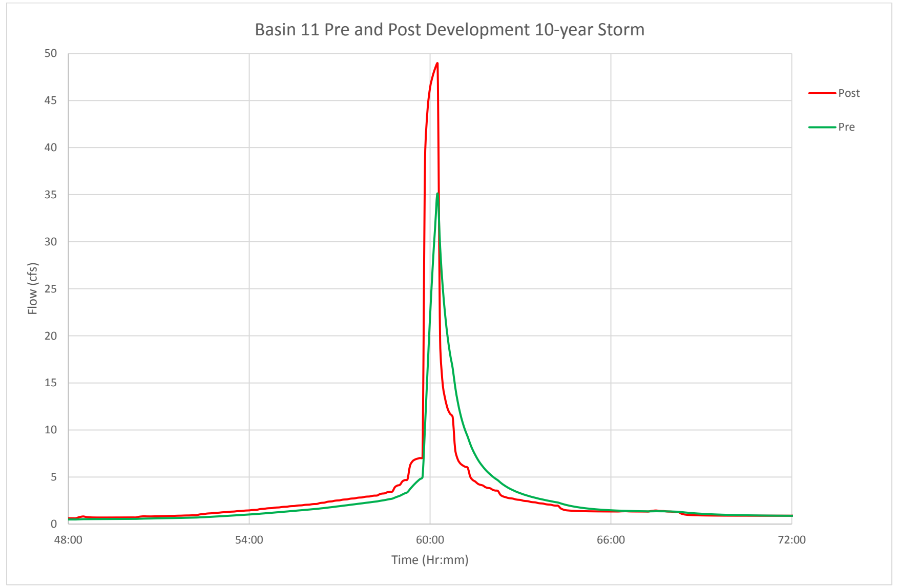
O.1 FIGURE: BASIN 11 PRE- AND POST-DEVELOPMENT HYDROGRAPH, 10-YEAR STORM
