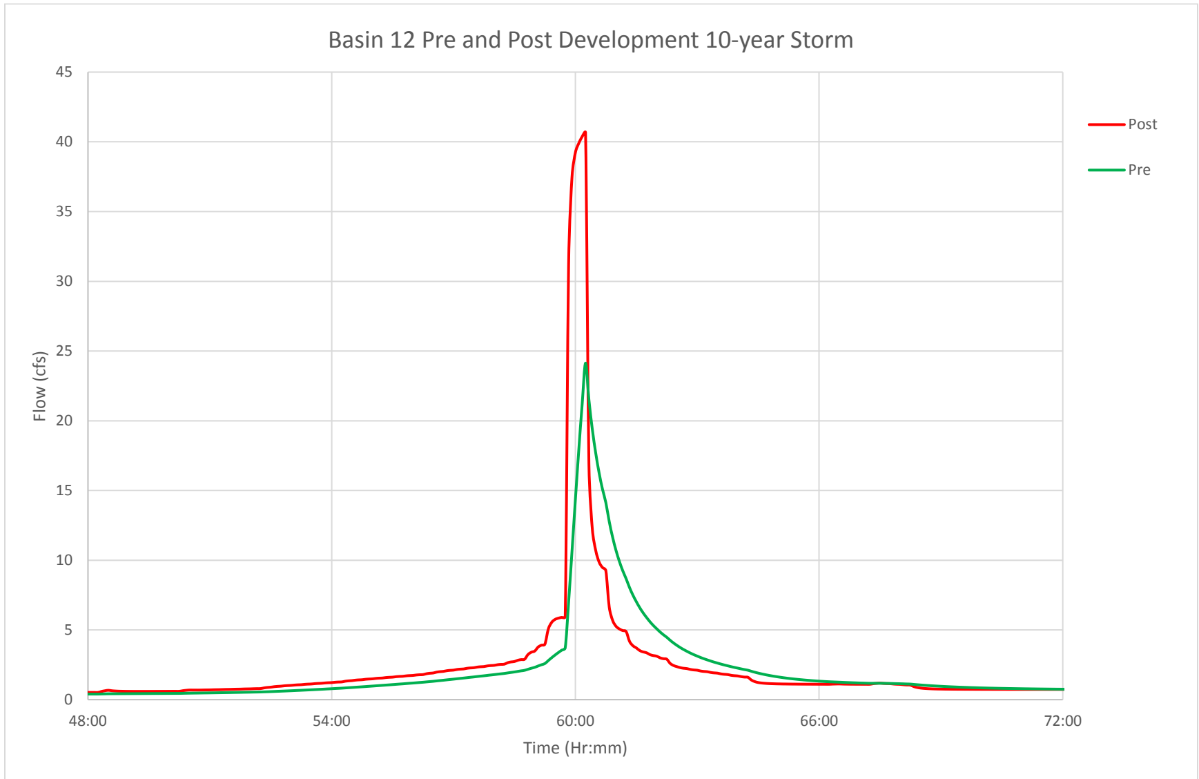
P.1 FIGURE: BASIN 12 PRE- AND POST-DEVELOPMENT HYDROGRAPH, 10-YEAR STORM
