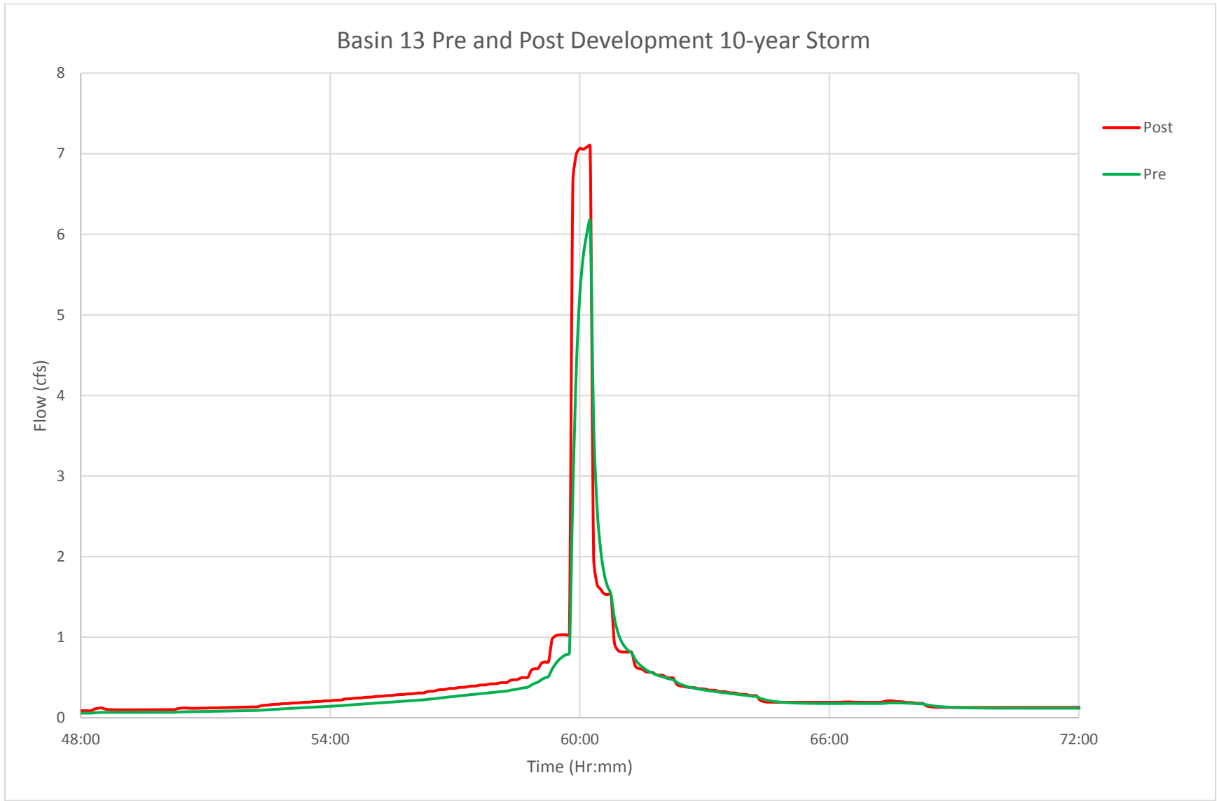
Q.1 FIGURE: BASIN 13 PRE- AND POST-DEVELOPMENT HYDROGRAPH, 10-YEAR STORM
