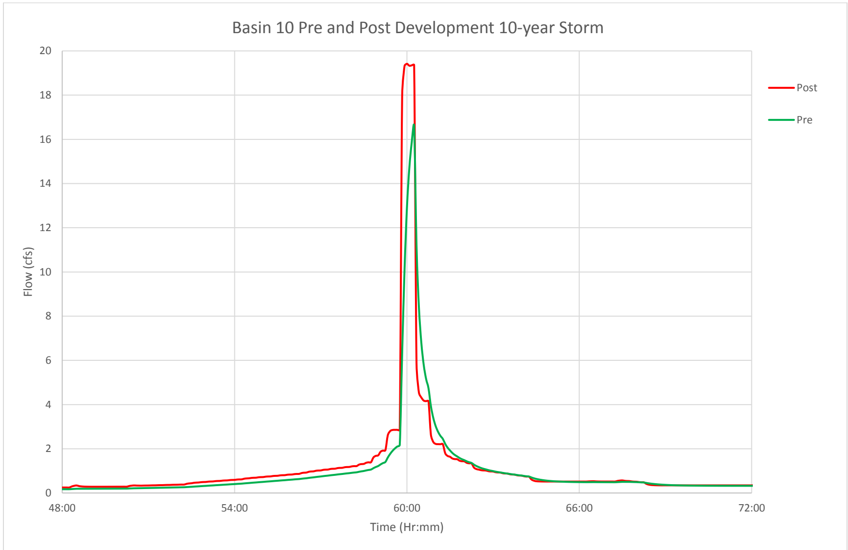
N.1 FIGURE: BASIN 10 PRE- AND POST-DEVELOPMENT HYDROGRAPH, 10-YEAR STORM
