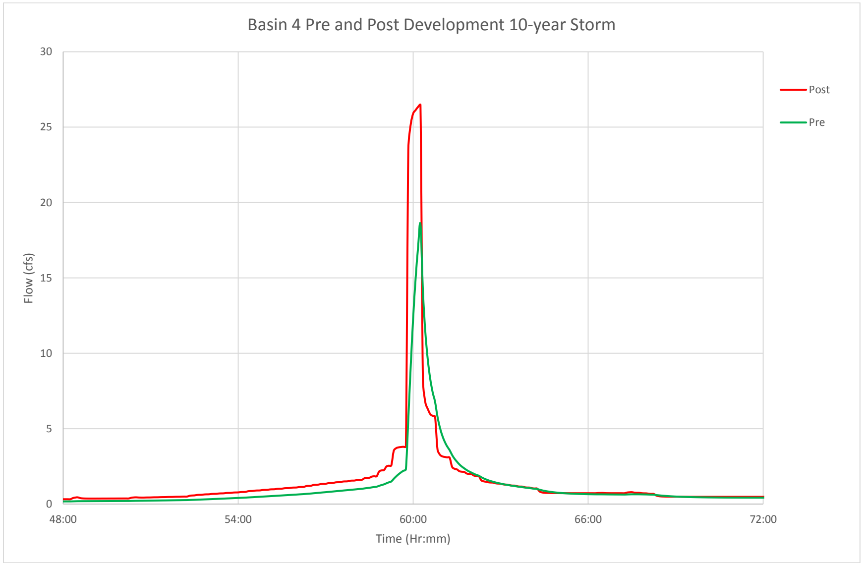
H.1 FIGURE: BASIN 4 PRE- AND POST-DEVELOPMENT HYDROGRAPH, 10-YEAR STORM
