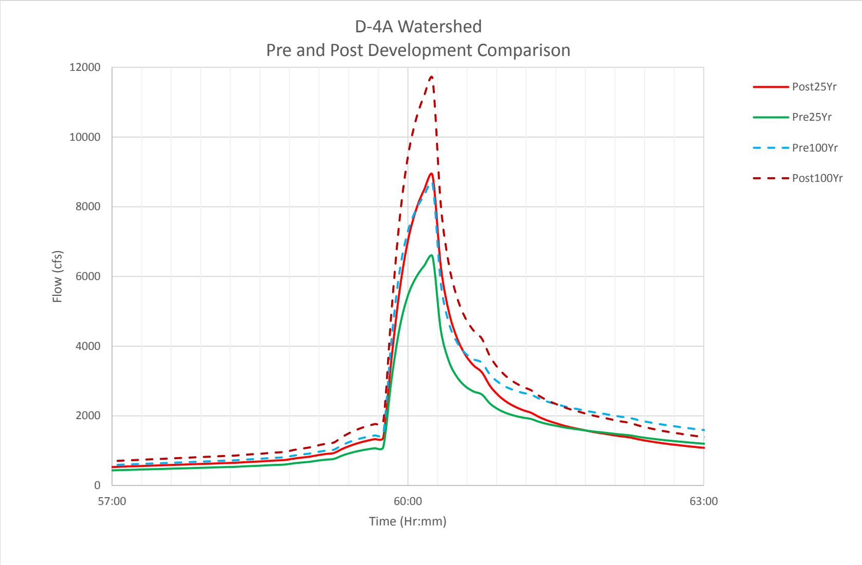
Figure 6.3 – Watershed D-4A Hydrograph
