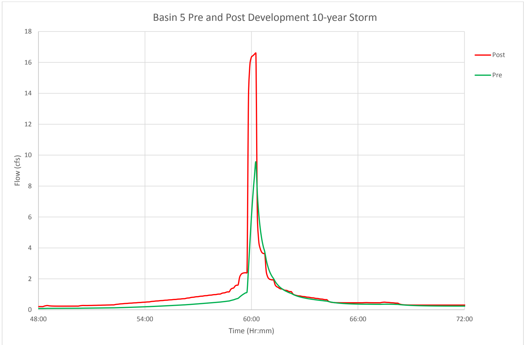
I.1 FIGURE: BASIN 5 PRE- AND POST-DEVELOPMENT HYDROGRAPH, 10-YEAR STORM
