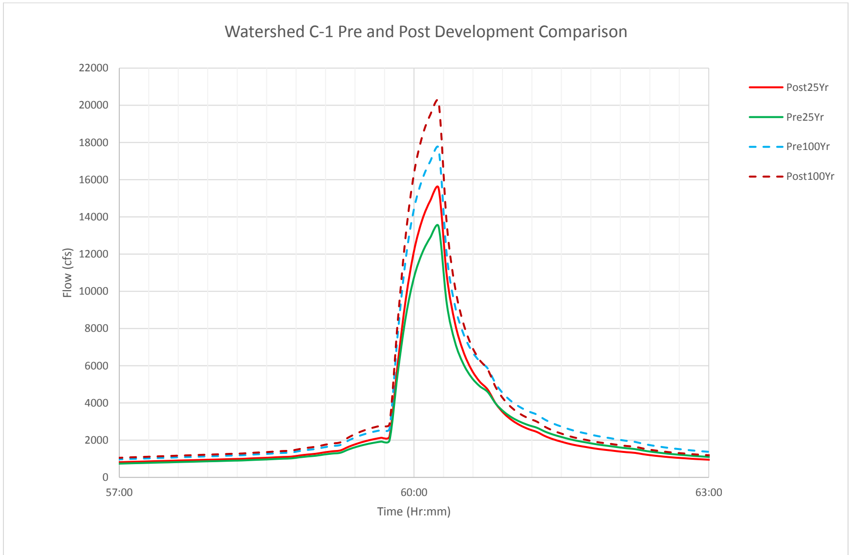
B.1 FIGURE: WATERSHED C-1 PRE- AND POST-DEVELOPMENT HYDROGRAPH
