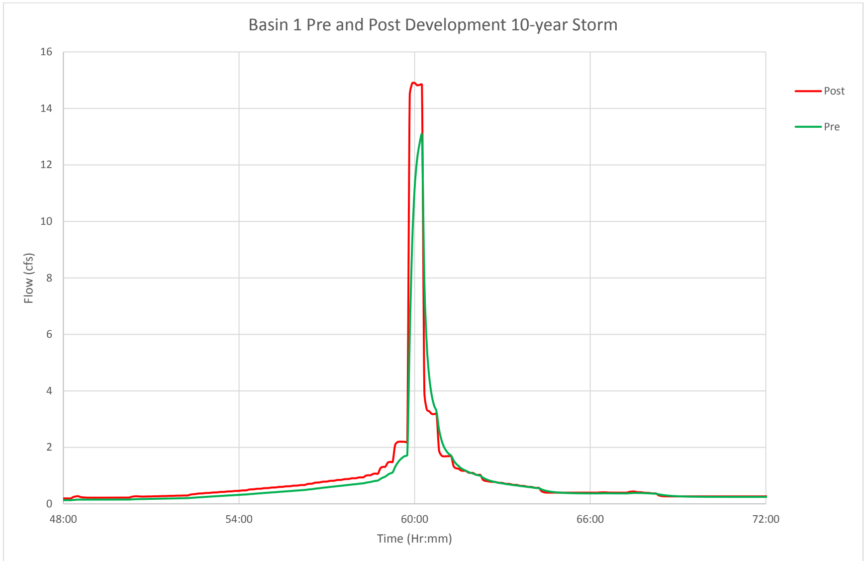
E.1 FIGURE: BASIN 1 PRE- AND POST-DEVELOPMENT HYDROGRAPH, 10-YEAR STORM
