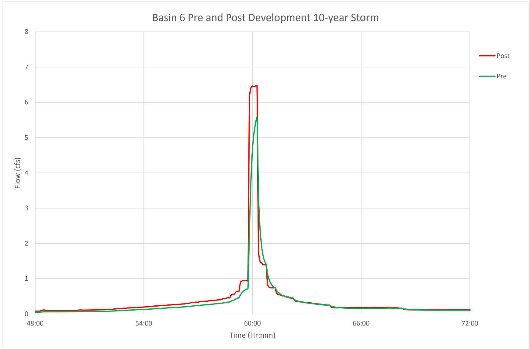
J.1 FIGURE: BASIN 6 PRE- AND POST-DEVELOPMENT HYDROGRAPH, 10-YEAR STORM
