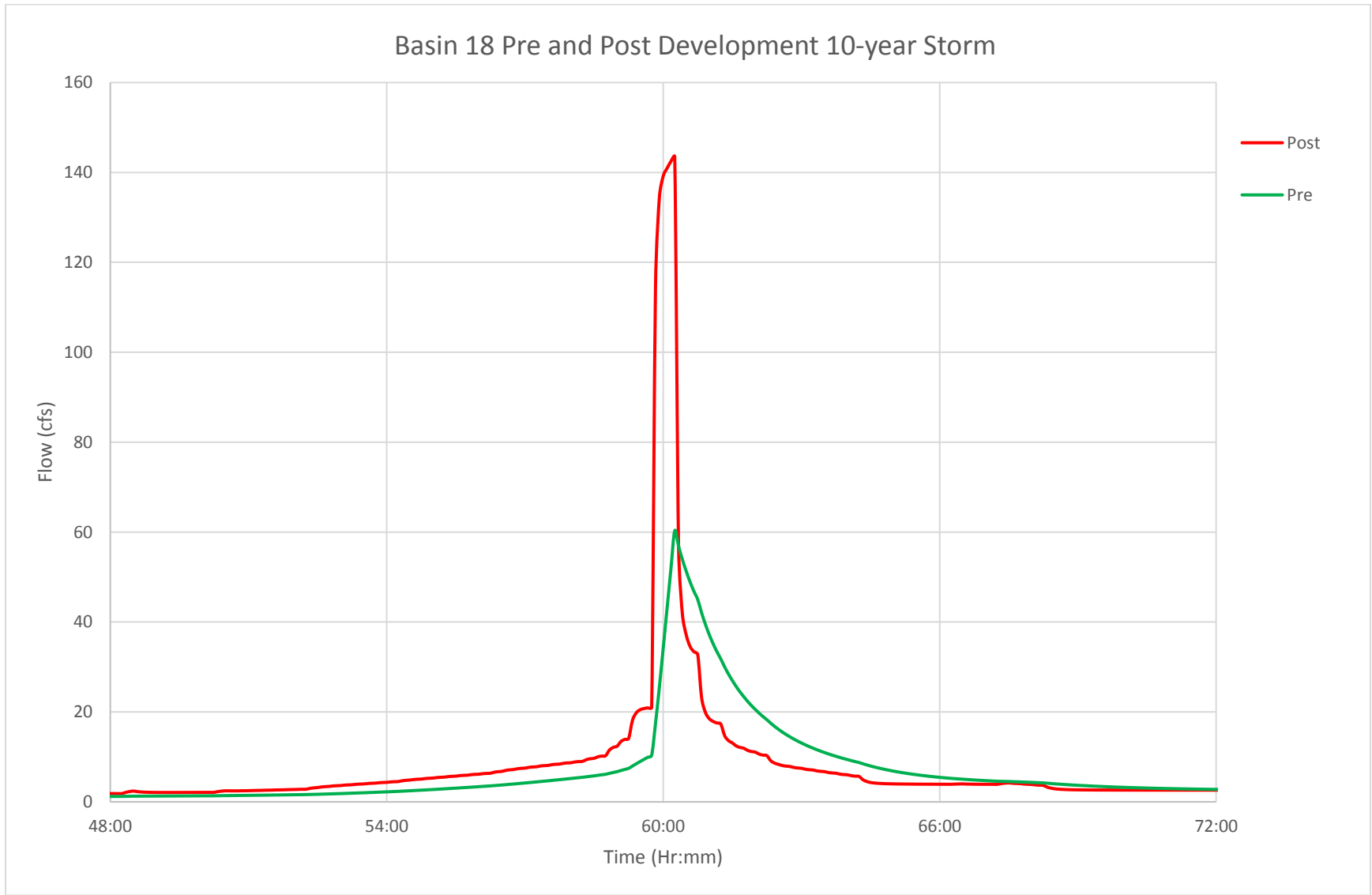
V.1 FIGURE: BASIN 18 PRE- AND POST-DEVELOPMENT HYDROGRAPH, 10-YEAR STORM
