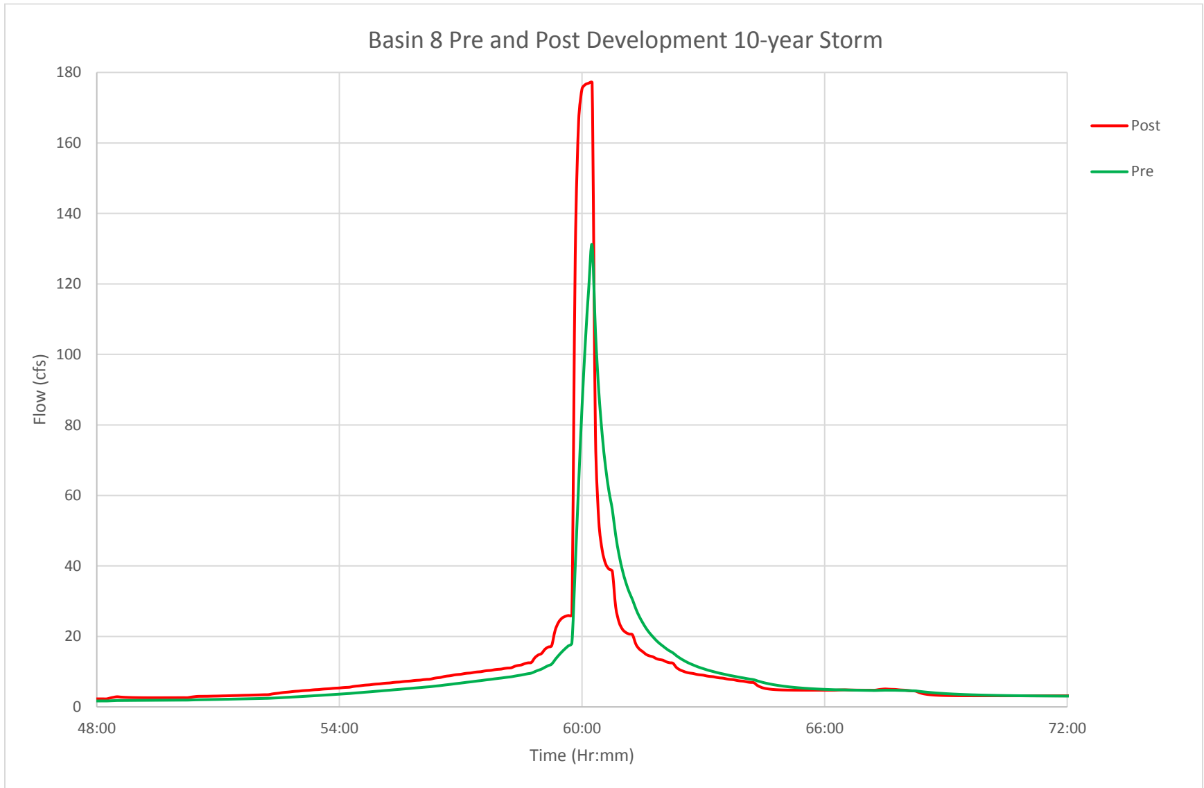
L.1 FIGURE: BASIN 8 PRE- AND POST-DEVELOPMENT HYDROGRAPH, 10-YEAR STORM
