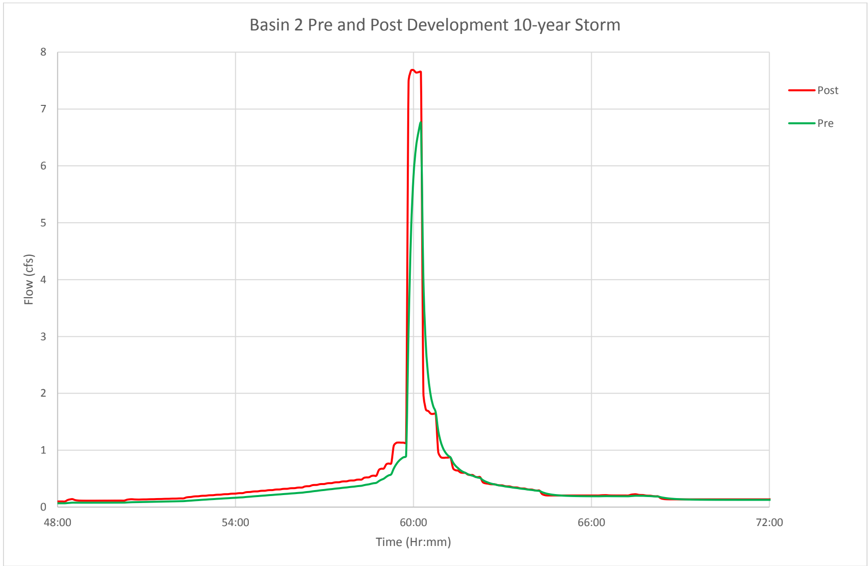
F.1 FIGURE: BASIN 2 PRE- AND POST-DEVELOPMENT HYDROGRAPH, 10-YEAR STORM
