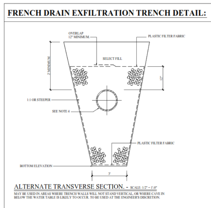
Figure 4.5.2. Exfiltration trench cross section
